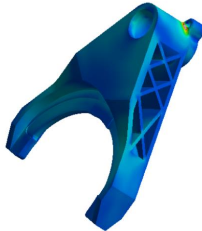
Optimized plastic design
